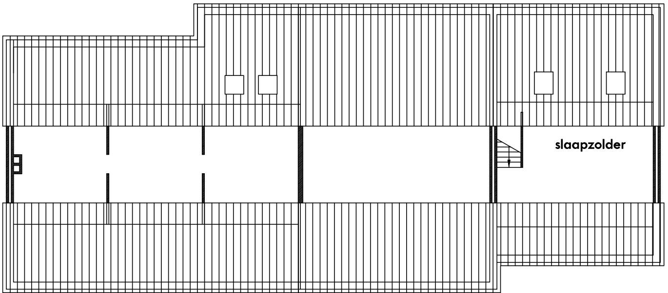
ZOLDER
